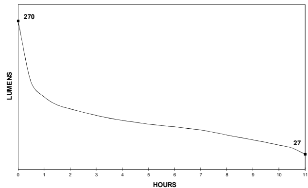
PERFORMANCE CURVE
